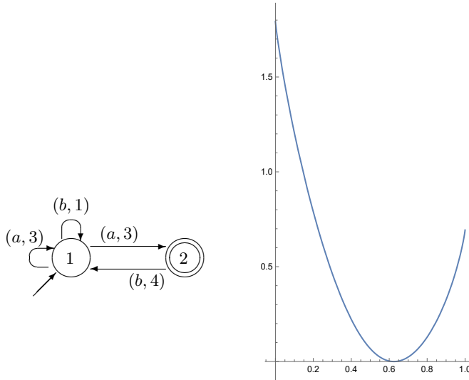
Fig. 1. Weighted finite automaton defining a sequence of r.v.'s \{Y_n\} with \lambda = 6 , \beta = 5/8 , \lambda_A = 3 , \lambda_B = 1 , and the graphic of the corresponding rate function I(x) .
